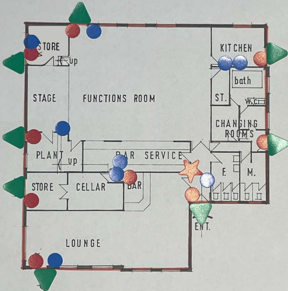
GROUND FLOOR PLAN Scale 1:200
