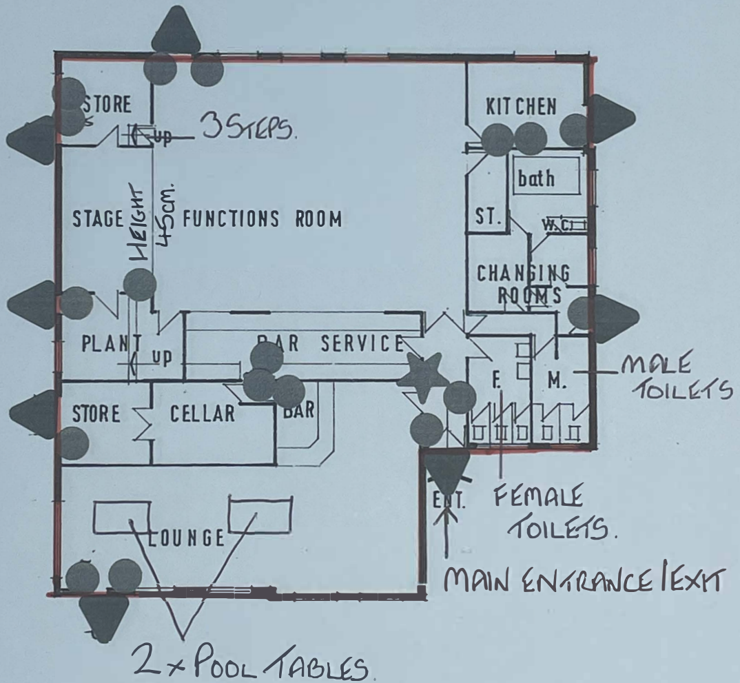
GROUND FLOOR PLAN Scale 1:200
